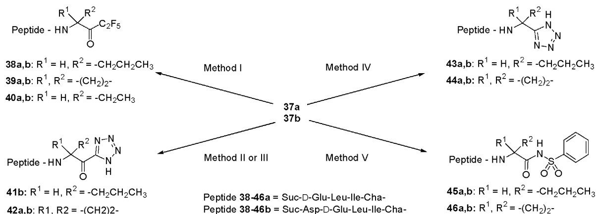
Scheme 6. Method I: (a) 10 , 11 or 12 , HATU, TMP; (b) 25% piperidine/DMF; (c) 2.5% TFA/ \text{CH}_2\text{Cl}_2 ; (d) Dess–Martin periodinane, (e) hv (350 nm), MeOH. Method II: (a) 21 , HATU, DIEA; (b) 25% piperidine/DMF; (c) 2.5% TFA/ \text{CH}_2\text{Cl}_2 ; (d) hv (350 nm), MeOH; (e) Dess–Martin periodinane. Method III: (a) 22 , HATU, DIEA; (b) 25% piperidine/DMF; (c) 2.5% TFA/ \text{CH}_2\text{Cl}_2 ; (d) Dess–Martin periodinane; (e) hv (350 nm), MeOH. Method IV: (a) 27 , 28 , HATU, DIEA; (b) 25% piperidine/DMF; (c) 2.5% TFA/ \text{CH}_2\text{Cl}_2 ; (d) hv (350 nm), MeOH. Method V: (a) 33 , 34 , HATU, TMP; (b) 25% piperidine/DMF, (c) 2.5% TFA/ \text{CH}_2\text{Cl}_2 , (d) hv (350 nm), MeOH.
