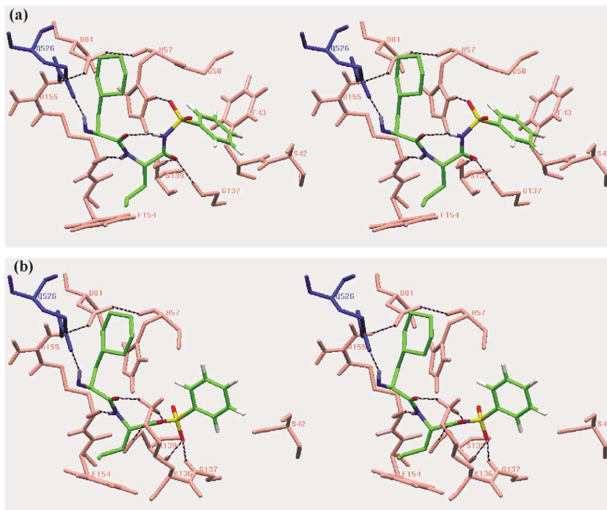
Figure 1. Stereoview of two possible binding modes ( a and b ) of Suc-D-Glu-Leu-Ile-Cha-Nva-NHSO 2 Ph 45a docked into the protease active site of the full-length scNS3-NS4A protein. Protease (3–181) residues depicted in pink, helicase (182–631) residues in blue, and the inhibitor (only the P2–P1 part of the inhibitor shown) color-coded with all carbons in green, oxygens in red, nitrogens in blue, and hydrogens in gray. Only residues close to the inhibitor (within 3.0 Å) are shown. Hydrogen bonds are indicated.
